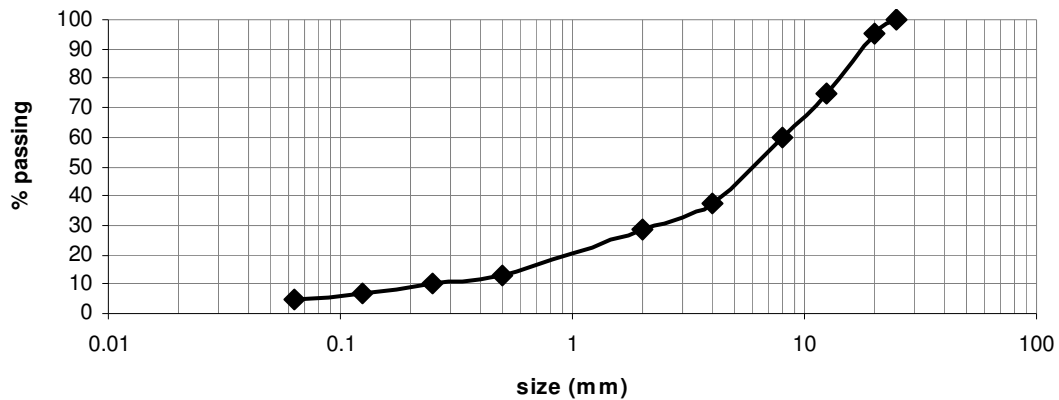
Figure2: Granulometric curve of the mixture AC 22 base G.
